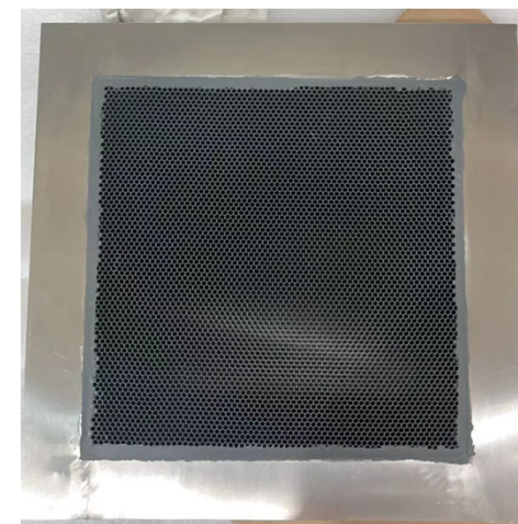
Stainless steel vent with L frame 3.2mm cell/25mm thickness 300x300mm core size
