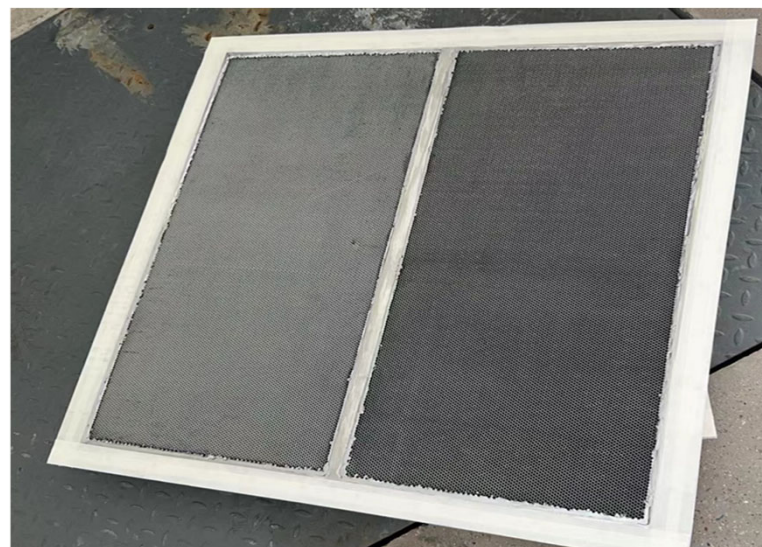
Stainless steel vent with L frame 3.2mm cell/25mm thickness 925x925mm size
