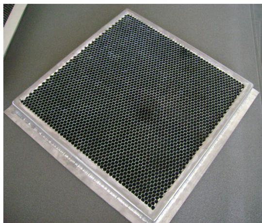
Steel vent with H frame 4.8mm cell/25mm thickness 300x300mm core size
