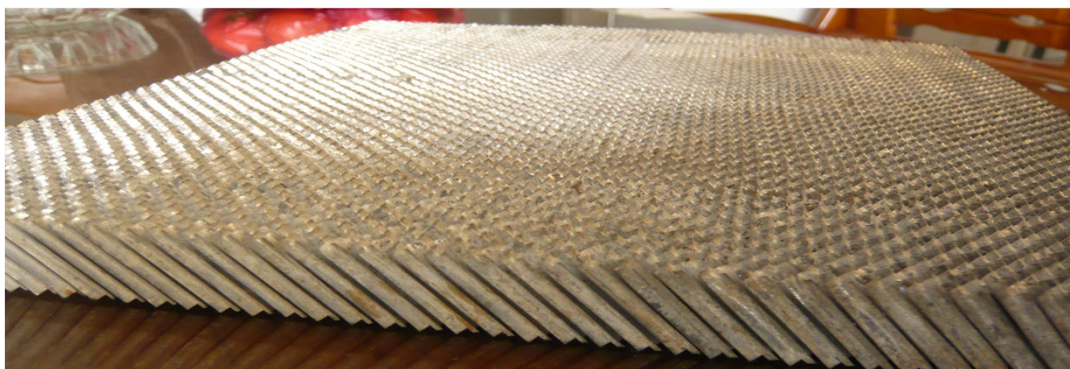
Stainless steel vent with L frame 4mm cell/25mm thickness 1150x1160mm size
